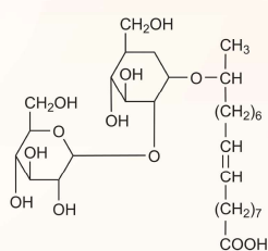
Acidic sophorolipid
