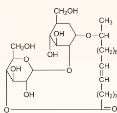
Lactonic sophorolipid
